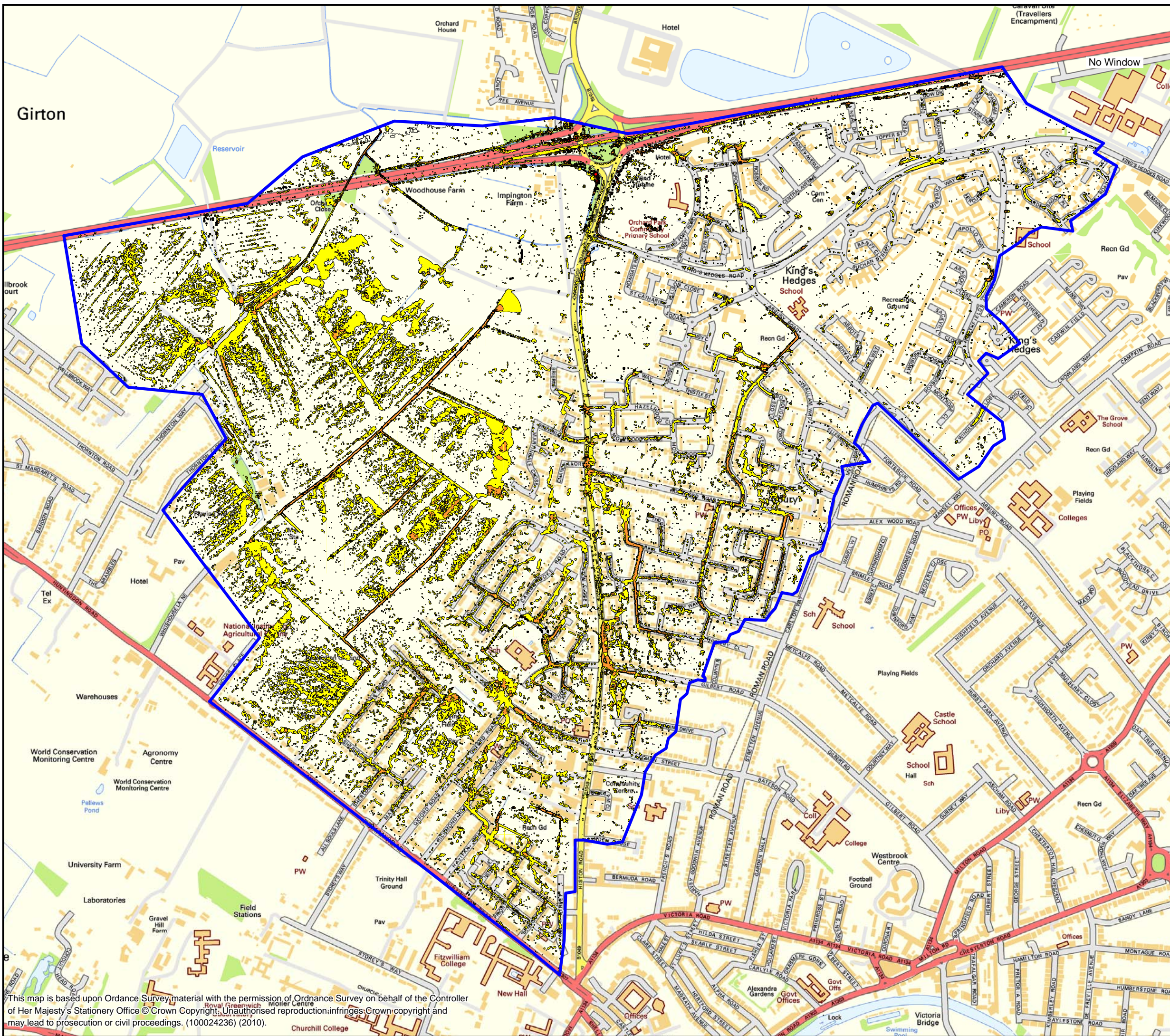
FIGURE F23 0.5% AEP "ENGINEERING OPTION C6" PLUVIAL MODELLING MAXIMUM VELOCITY - KING'S HEDGES AND ARBURY
